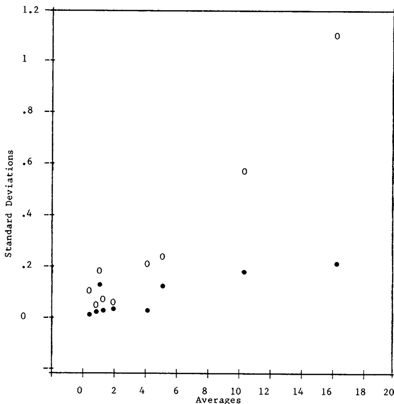
FIG. 9 Pentosans in Pulp: Standard Deviations of Reproducibility (○) and Repeatability (●) Versus Average
